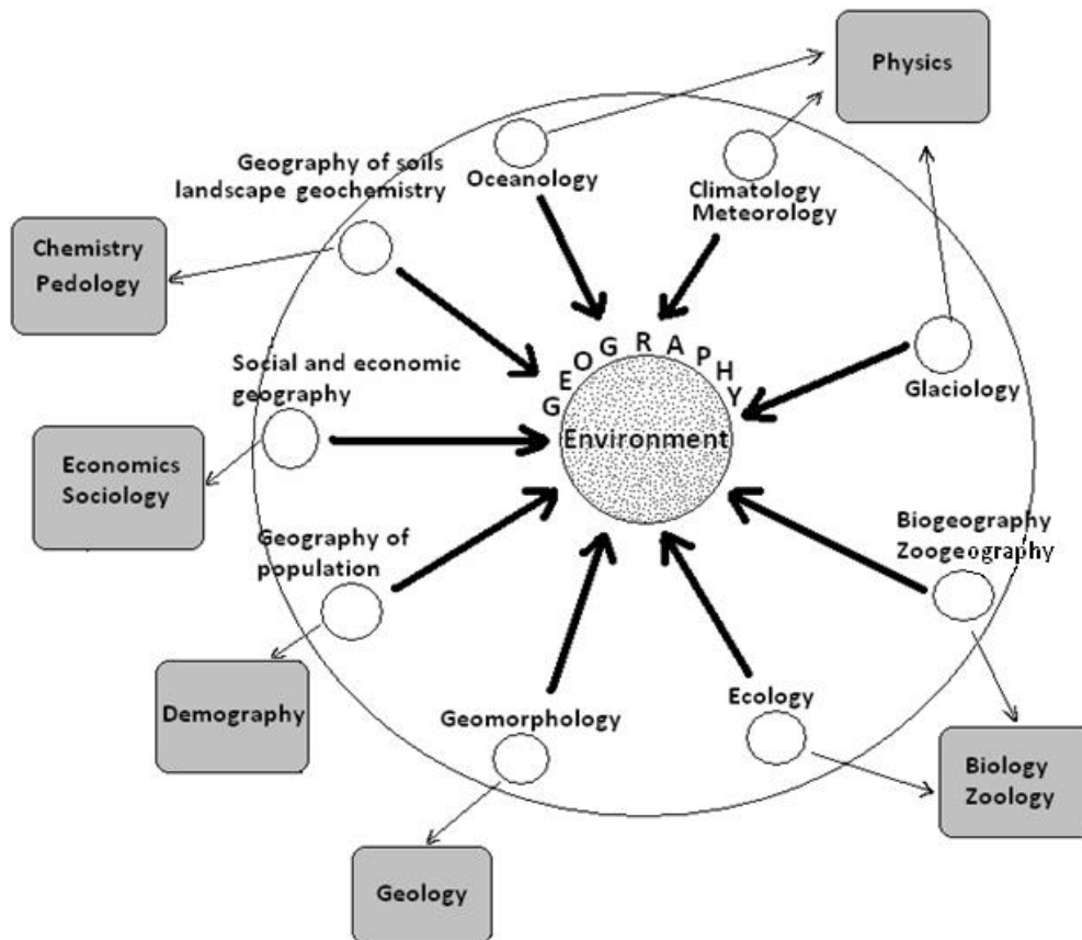
Figure 2. The place of geography and related sciences.
